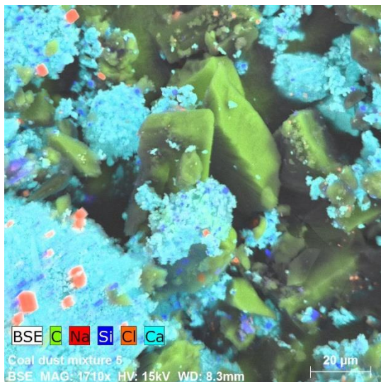
Element map of coal dust
